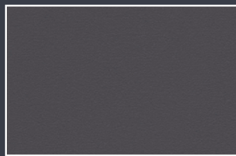
Graphite
